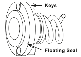
Keyed Floating Seal
